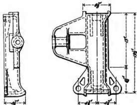
Figs. 4385-4387. Combined Column Casting and Brake Hanger Carrier.
